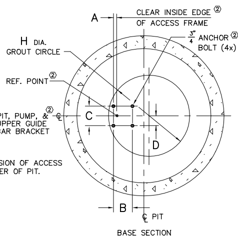
BASE SECTION
