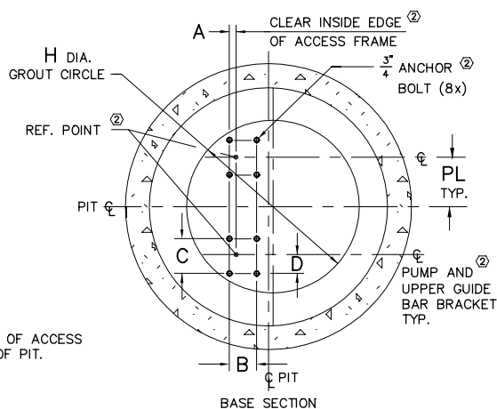
BASE SECTION
